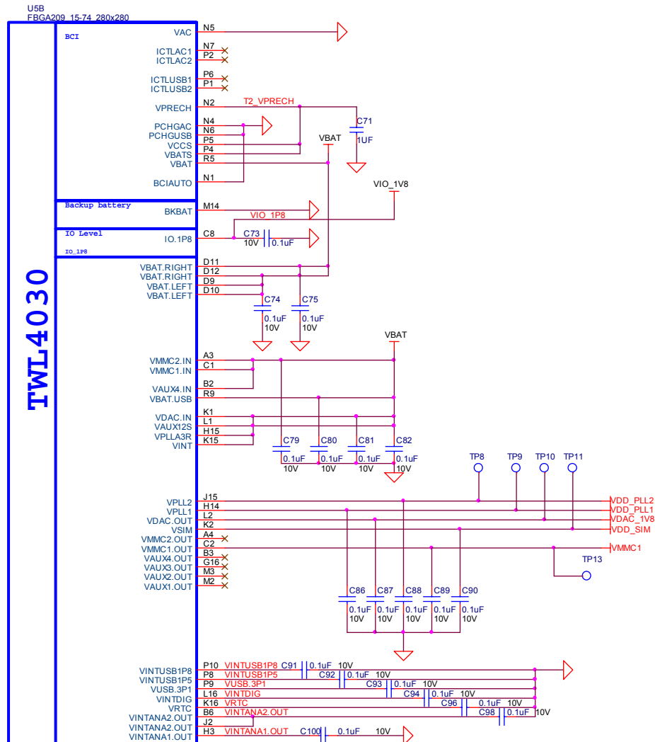
Figure 22. Peripheral Voltages
