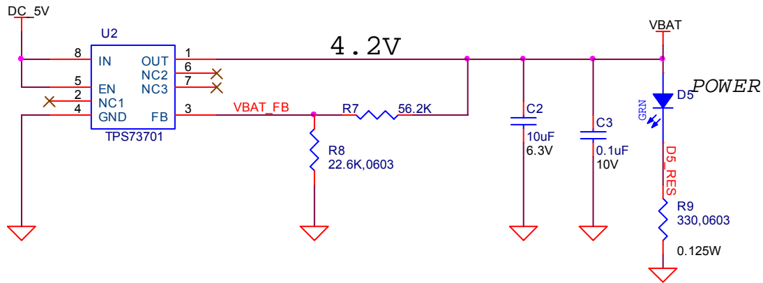
Figure 20. Power Conditioning
