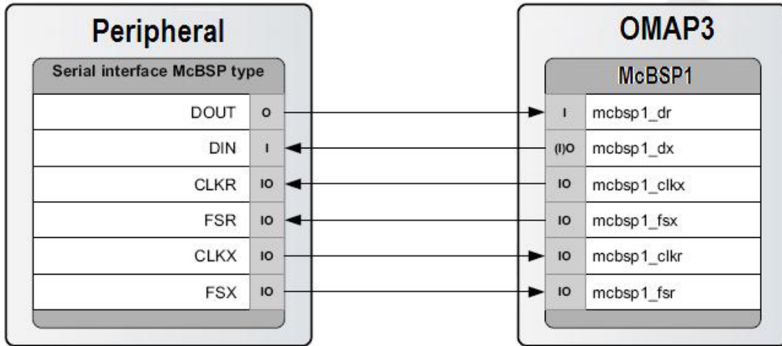
Figure 27. McBSP1 Interface
