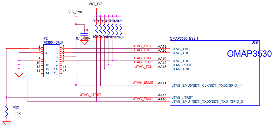
Figure 41. JTAG Interface
