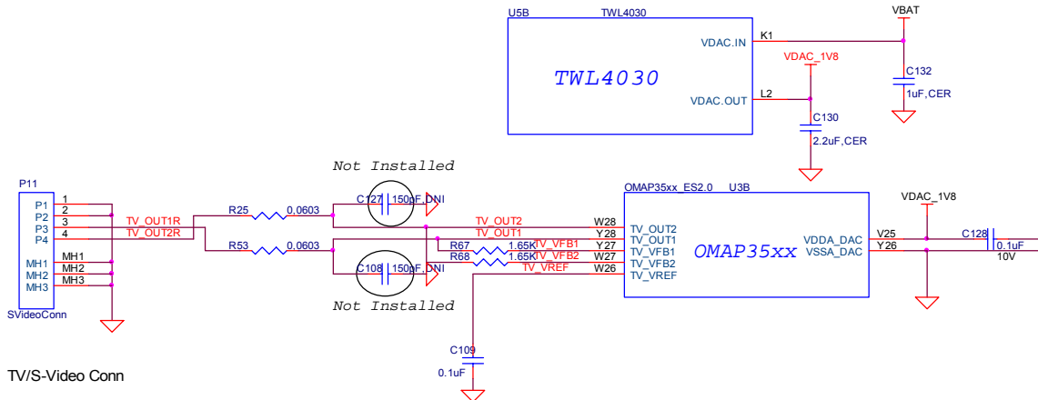
Figure 37. S-Video Interface
