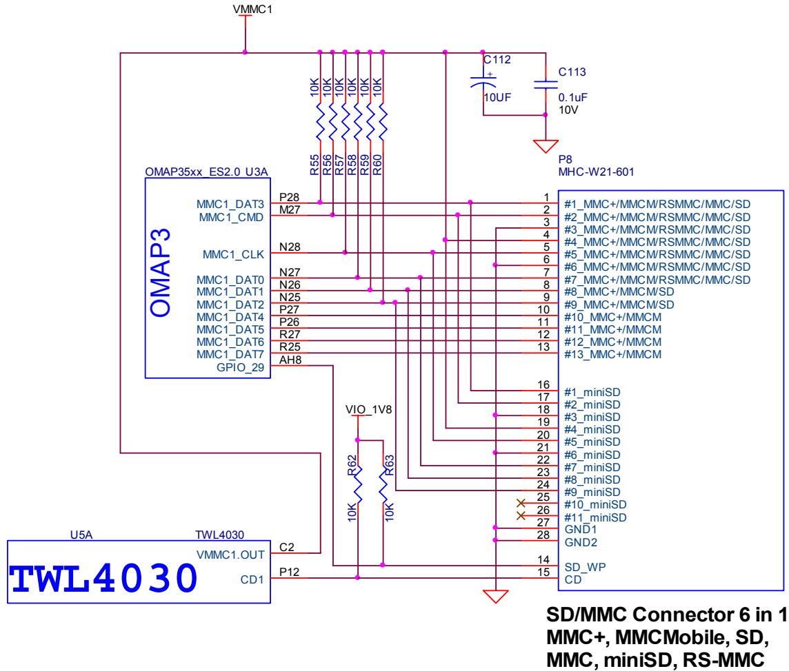
Figure 34. SD/MMC Interface
