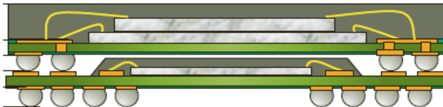
Figure 29. POP Memory
