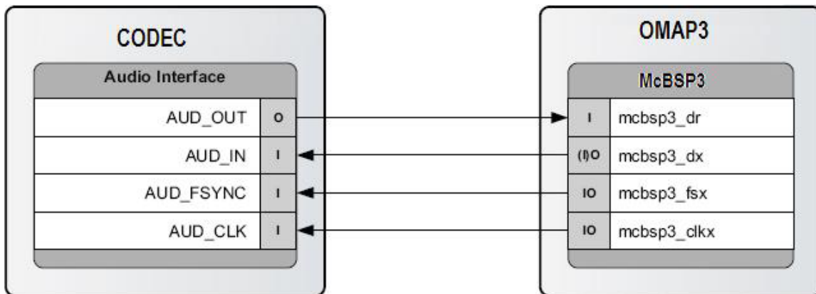
Figure 28. McBSP3 Interface
